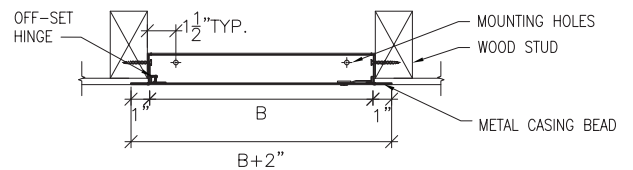
Section Detail
