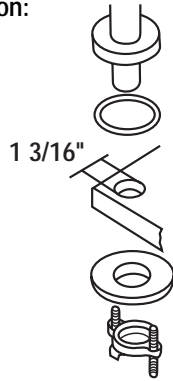
Drill 1 3/16" for the inlet
