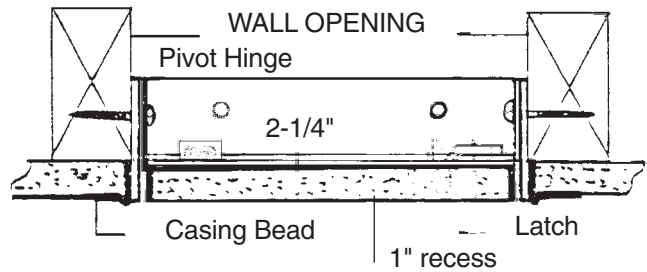
SECTION DETAIL
