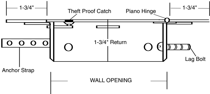
SECTION DETAIL
