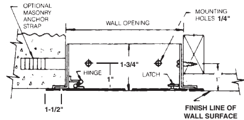
SECTION DETAIL
